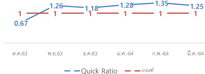
QUICK RATIO
