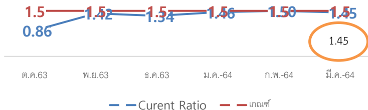
CURRENT RATIO
