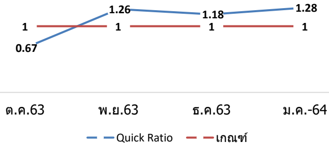
QUICK RATIO
